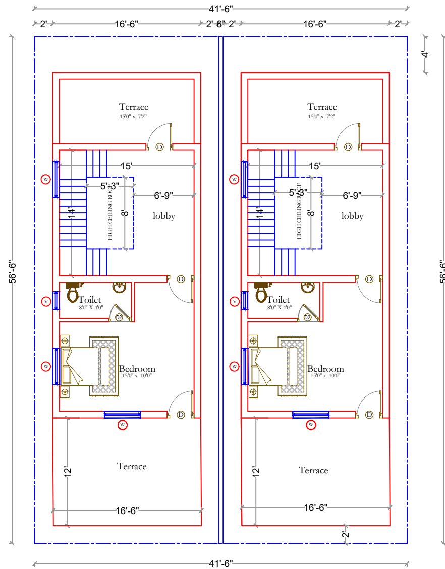
FIRST FLOOR PLAN - 504 Sq.ft/ house
