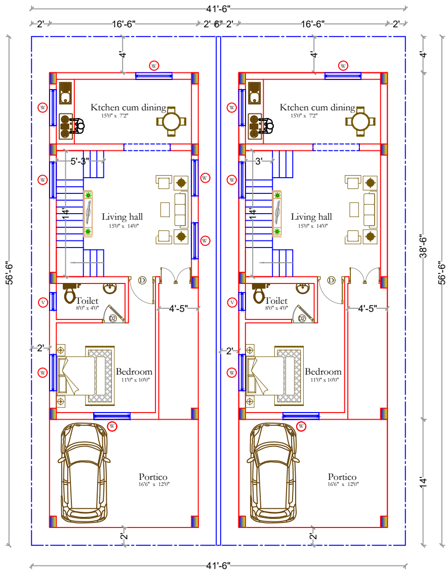
GROUND FLOOR PLAN - 833.48 Sq.ft /house
